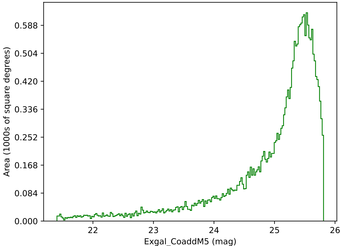
ddf_acor_sf10_lsf20_lsr10_v3.4_10yrs Yr 1 g band: Exgal_CoaddM5
