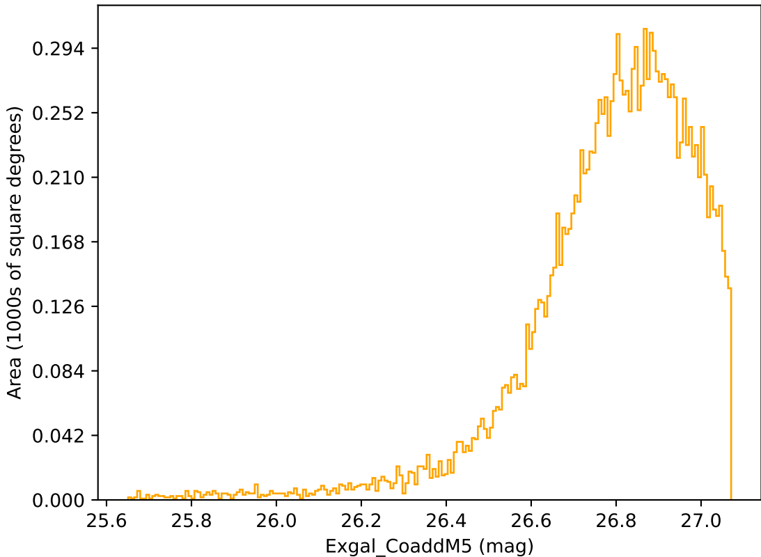
ddf_acor_sf10_lsf20_lsr10_v3.4_10yrs WFD r band: Exgal_CoaddM5
