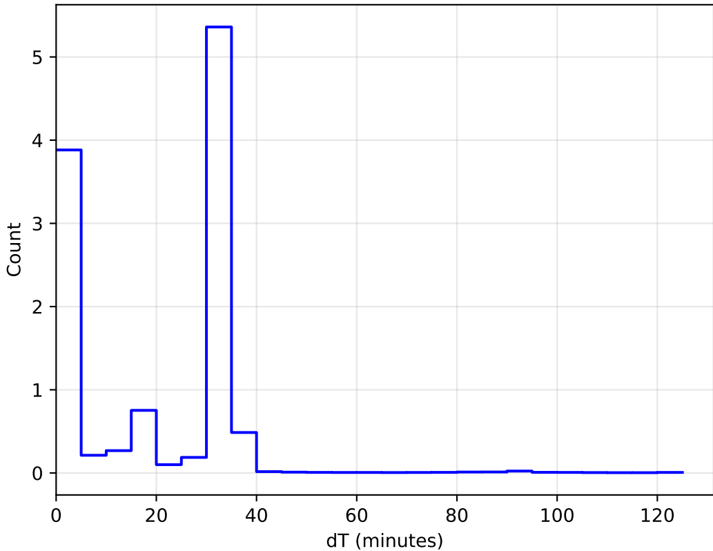
ddf_acor_sf10_lsf20_lsr10_v3.4_10yrs WFD: DeltaT Histogram 1e6
