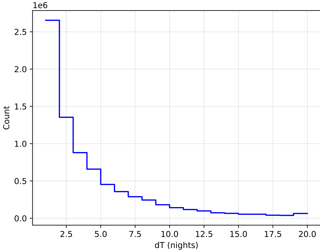
ddf_acor_sf10_lsf20_lsr10_v3.4_10yrs WFD all bands: DeltaNight Histogram
