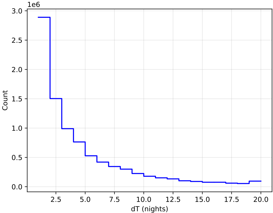
ddf_acor_sf10_lsf20_lsr10_v3.4_10yrs All sky all bands: DeltaNight Histogram
