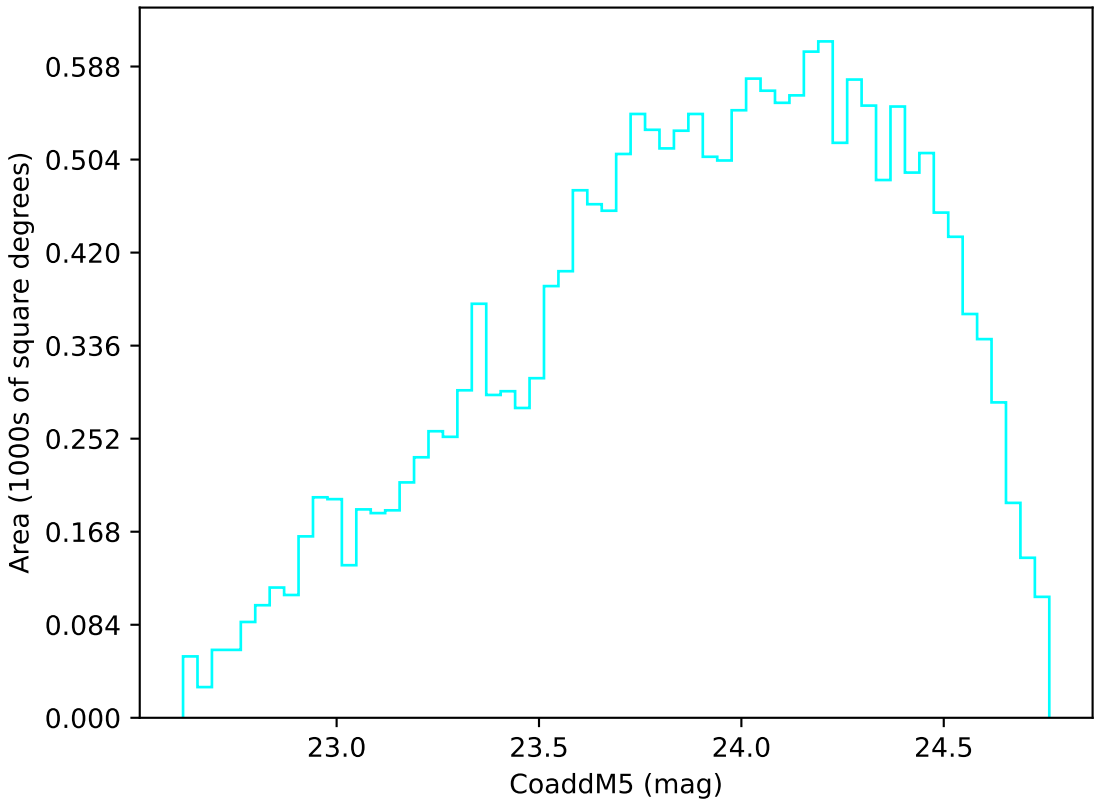
ddf_acor_sf10_lsf20_lsr10_v3.4_10yrs Yr 3-4 u band: CoaddM5
