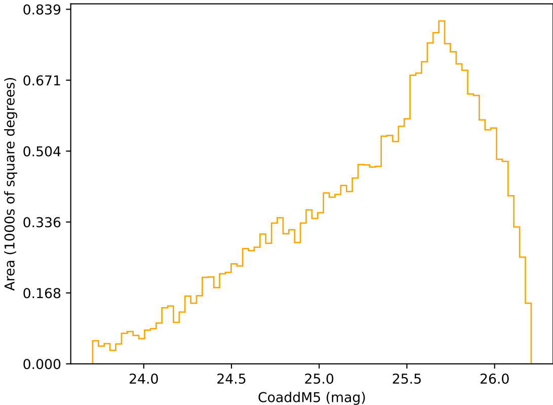
ddf_acor_sf10_lsf20_lsr10_v3.4_10yrs Yr 3-4 r band: CoaddM5
