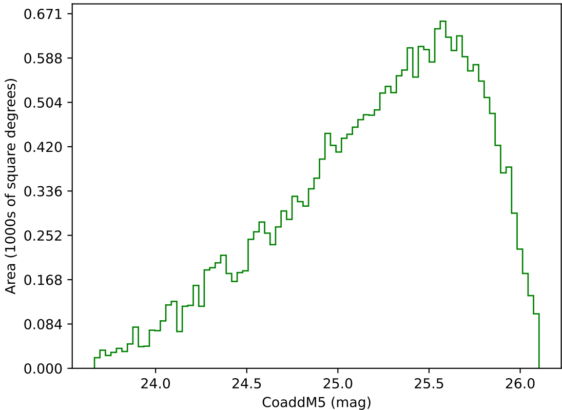
ddf_acor_sf10_lsf20_lsr10_v3.4_10yrs Yr 3-4 g band: CoaddM5
