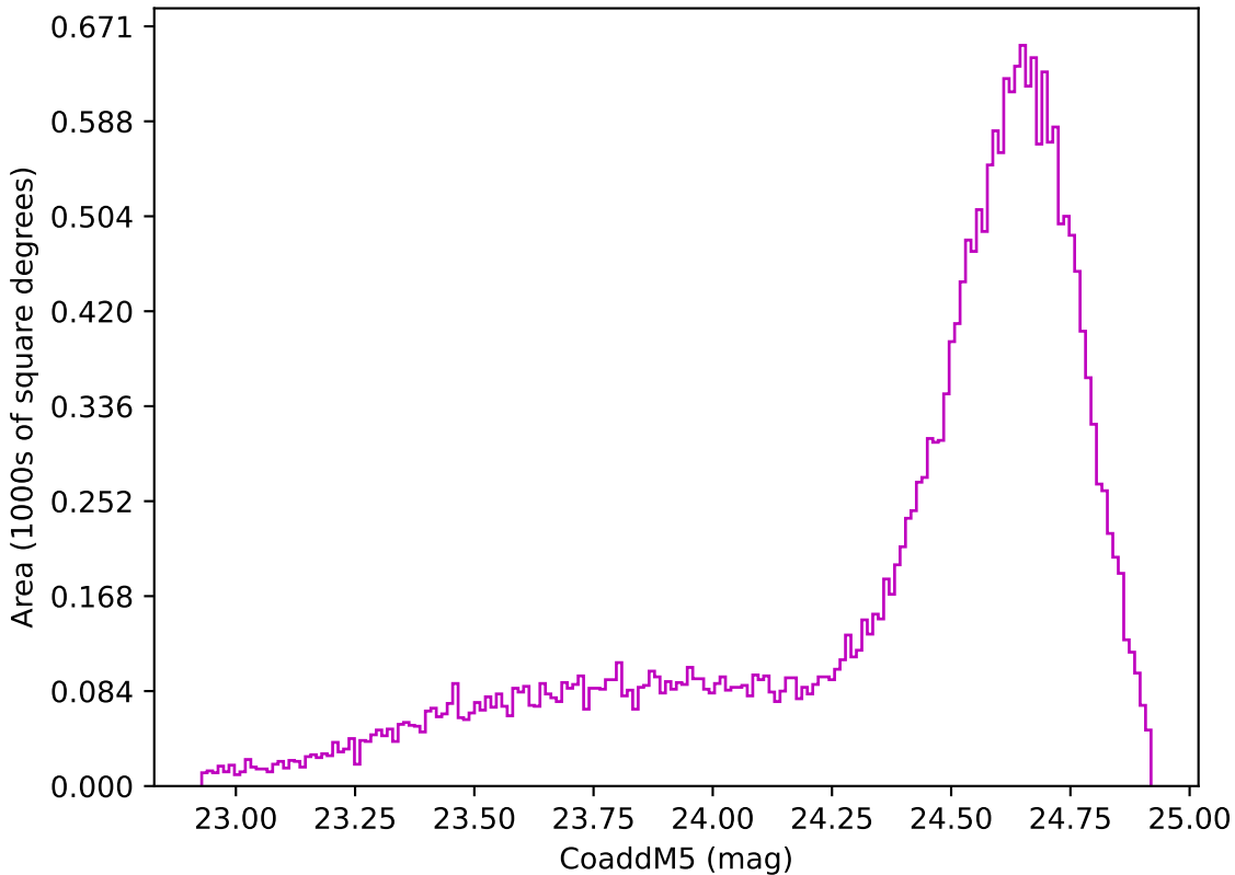
ddf_acor_sf10_lsf20_lsr10_v3.4_10yrs Yr 1 z band: CoaddM5
