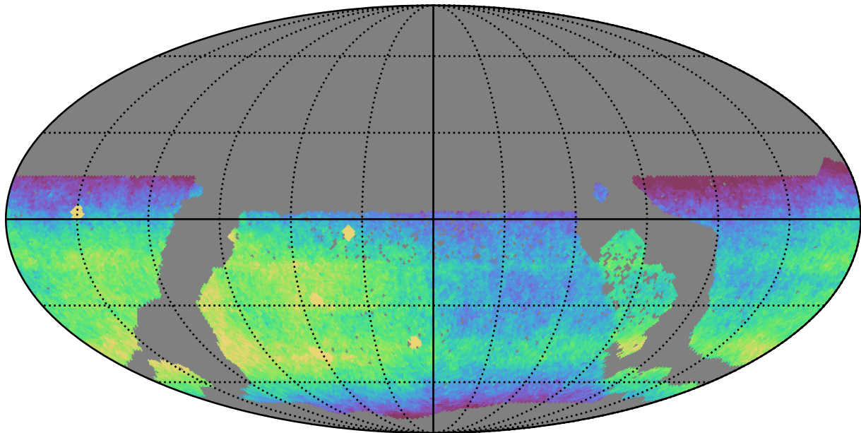
ddf_acor_sf10_lsf20_lsr10_v3.4_10yrs WFD r band: CoaddM5
