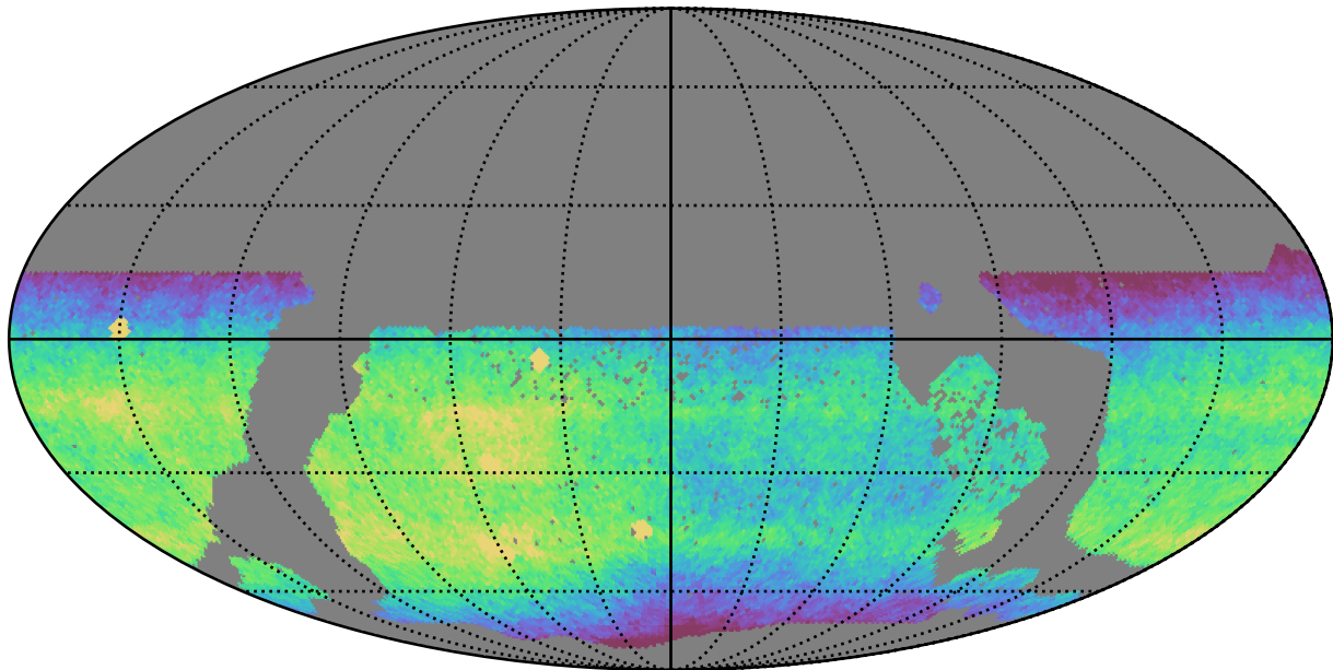
ddf_acor_sf10_lsf20_lsr10_v3.4_10yrs WFD i band: CoaddM5
