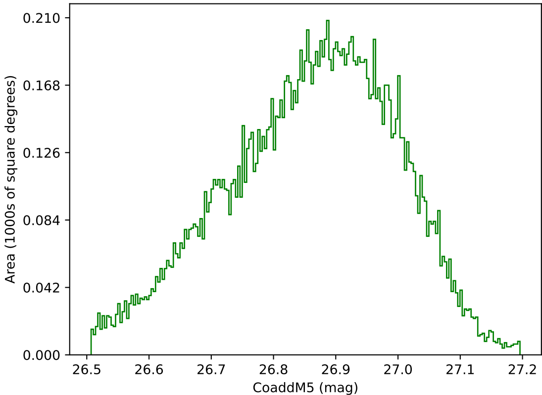
ddf_acor_sf10_lsf20_lsr10_v3.4_10yrs WFD g band: CoaddM5
