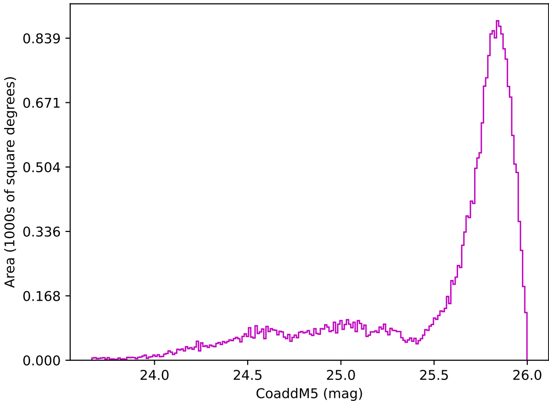
ddf_acor_sf10_lsf20_lsr10_v3.4_10yrs All sky z band: CoaddM5
