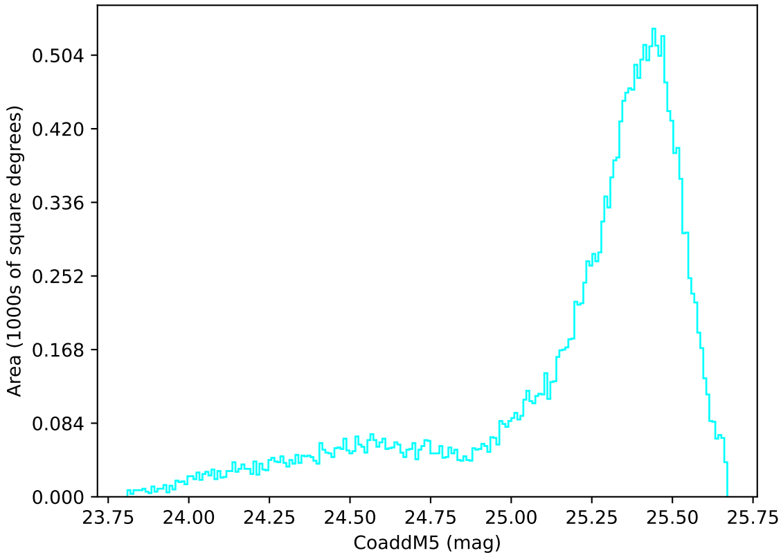
ddf_acor_sf10_lsf20_lsr10_v3.4_10yrs All sky u band: CoaddM5
