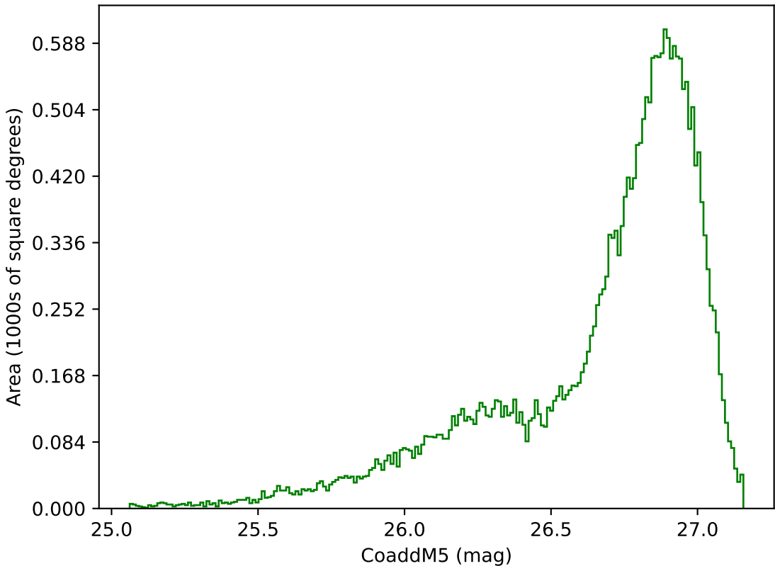
ddf_acor_sf10_lsf20_lsr10_v3.4_10yrs All sky g band: CoaddM5
