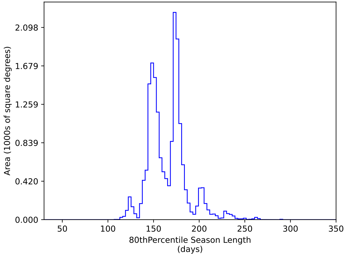
ddf_acor_sf10_lsf20_lsr10_v3.4_10yrs WFD y band: 80thPercentile Season Length
