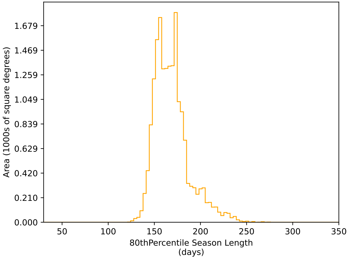
ddf_acor_sf10_lsf20_lsr10_v3.4_10yrs WFD r band: 80thPercentile Season Length
