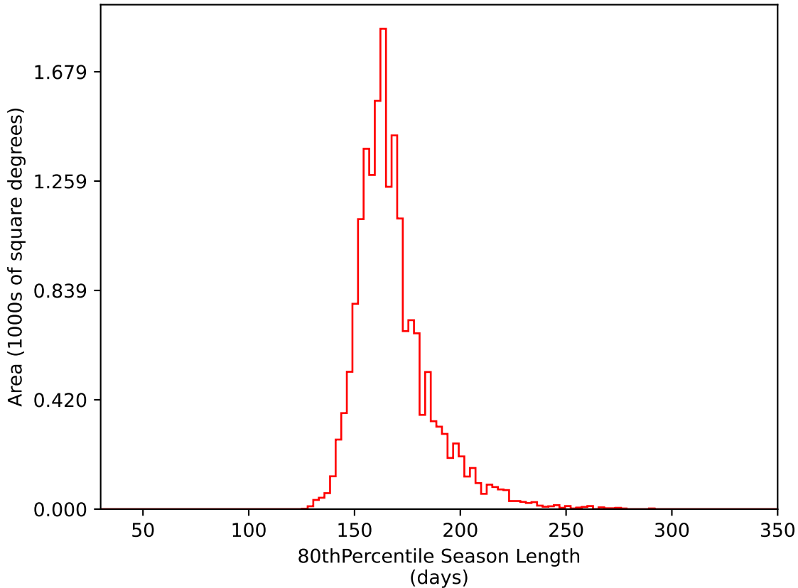
ddf_acor_sf10_lsf20_lsr10_v3.4_10yrs WFD i band: 80thPercentile Season Length
