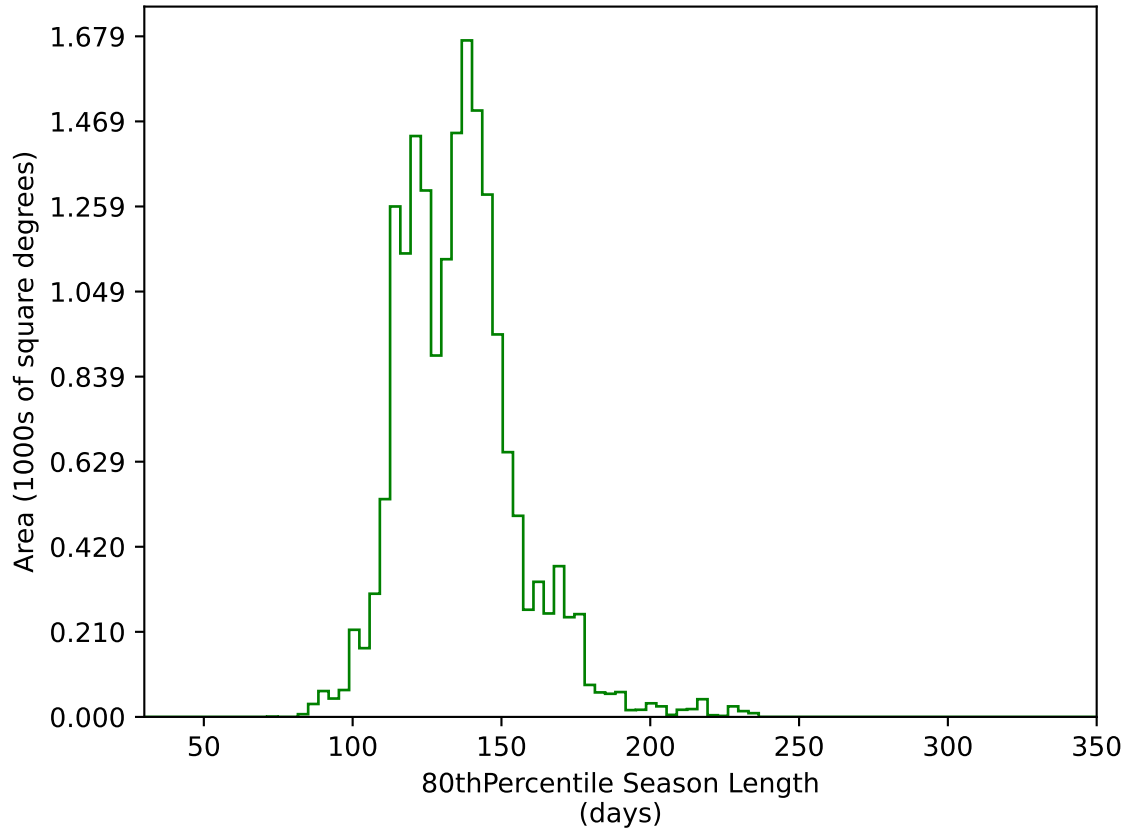
ddf_acor_sf10_lsf20_lsr10_v3.4_10yrs WFD g band: 80thPercentile Season Length
