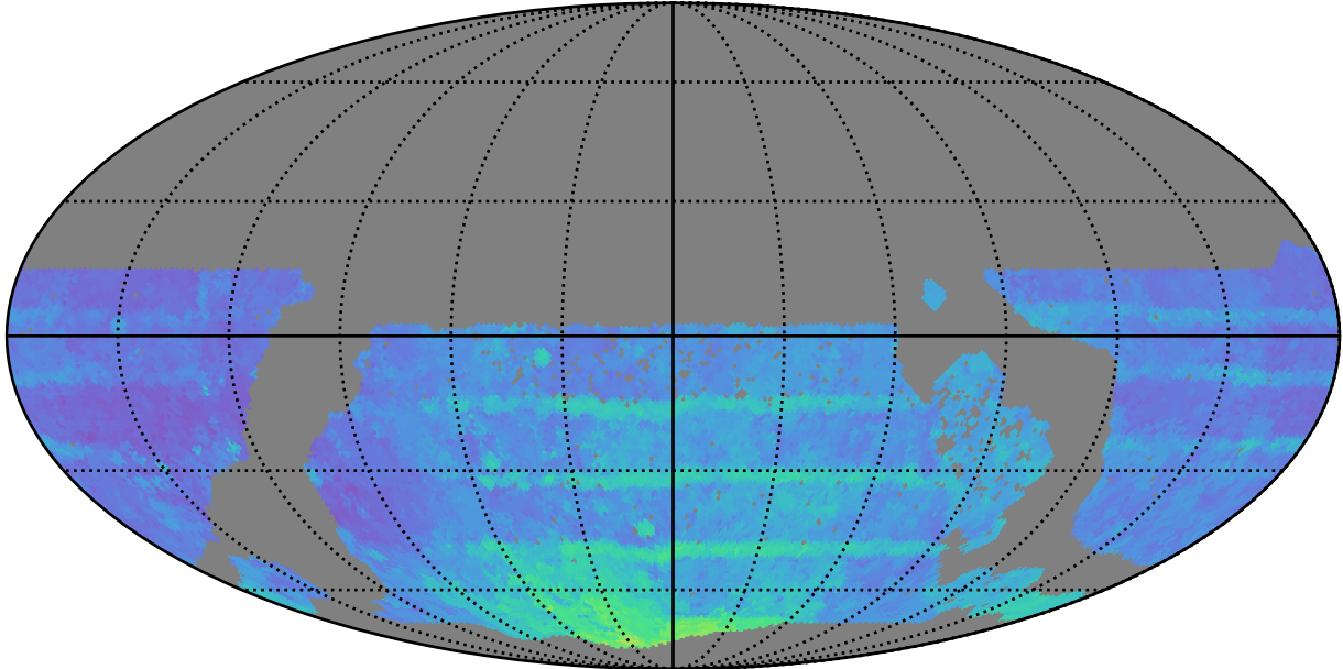
ddf_acor_sf10_lsf20_lsr10_v3.4_10yrs WFD all bands: 80thPercentile Season Length
