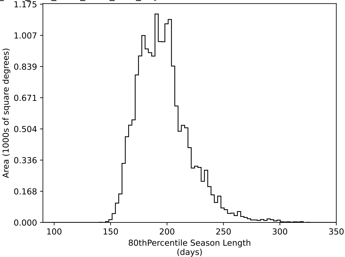
ddf_acor_sf10_lsf20_lsr10_v3.4_10yrs WFD all bands: 80thPercentile Season Length
