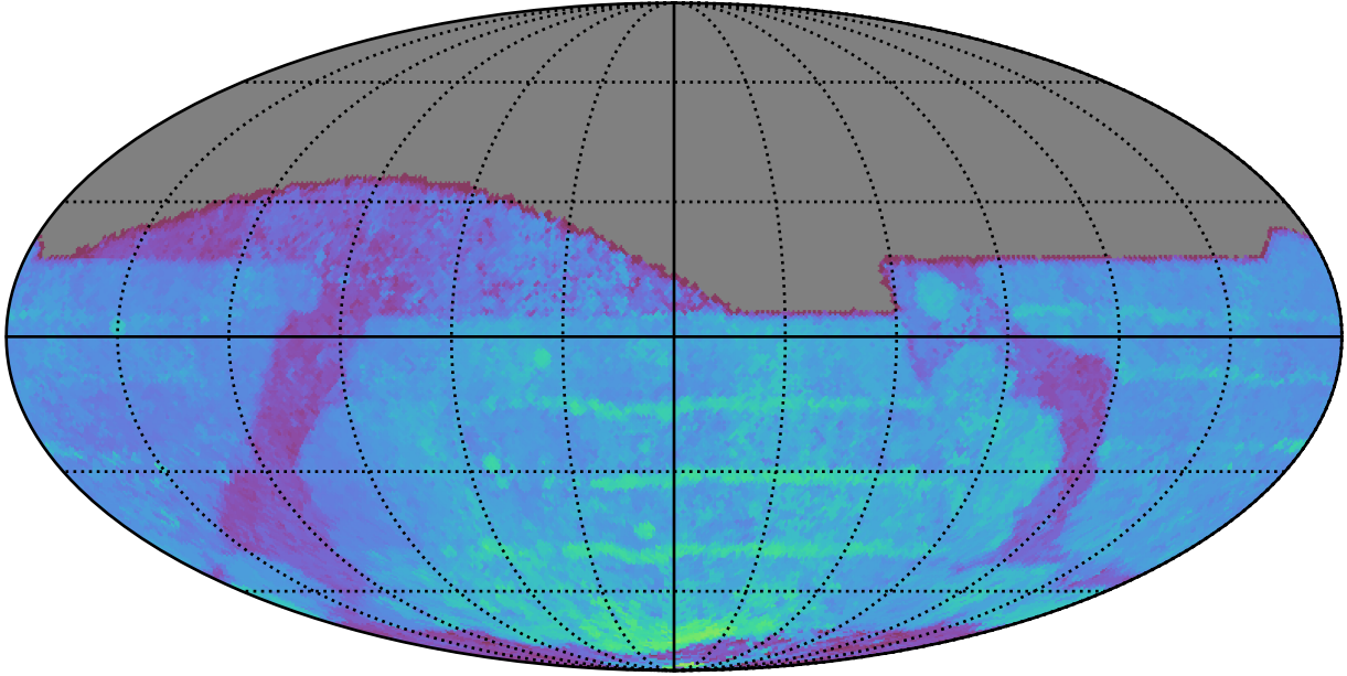
ddf_acor_sf10_lsf20_lsr10_v3.4_10yrs All sky z band: 80thPercentile Season Length
