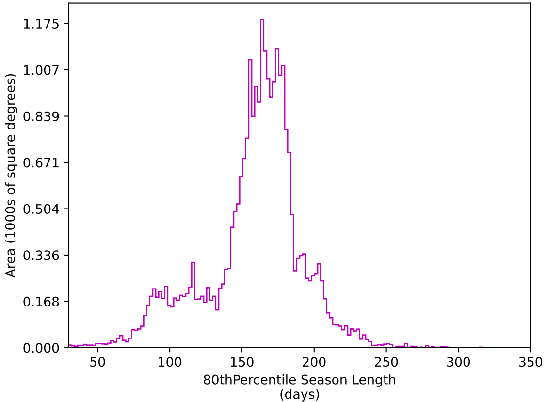
ddf_acor_sf10_lsf20_lsr10_v3.4_10yrs All sky z band: 80thPercentile Season Length
