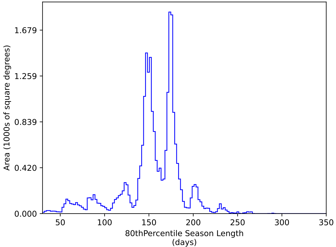
ddf_acor_sf10_lsf20_lsr10_v3.4_10yrs All sky y band: 80thPercentile Season Length
