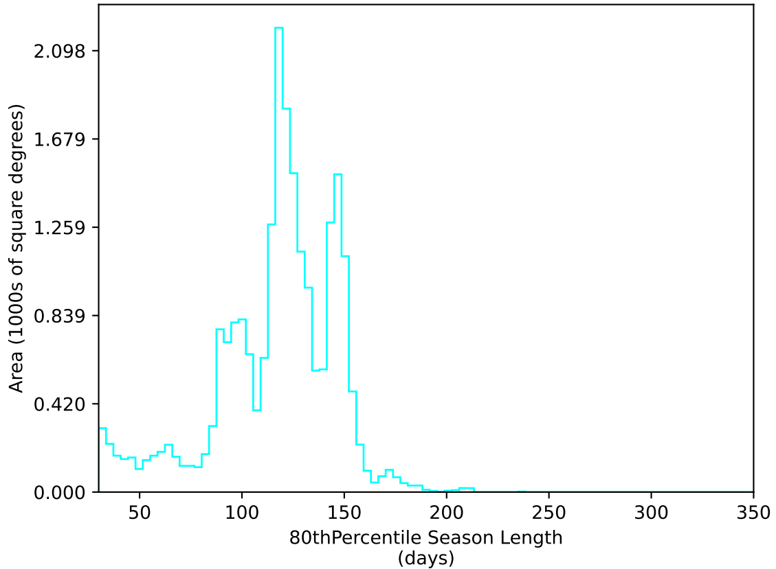
ddf_acor_sf10_lsf20_lsr10_v3.4_10yrs All sky u band: 80thPercentile Season Length
