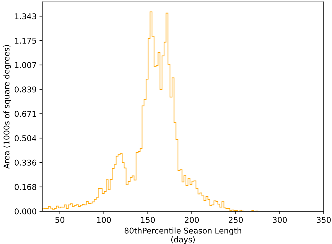
ddf_acor_sf10_lsf20_lsr10_v3.4_10yrs All sky r band: 80thPercentile Season Length
