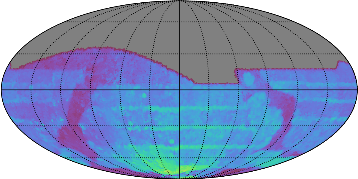
ddf_acor_sf10_lsf20_lsr10_v3.4_10yrs All sky all bands: 80thPercentile Season Length
