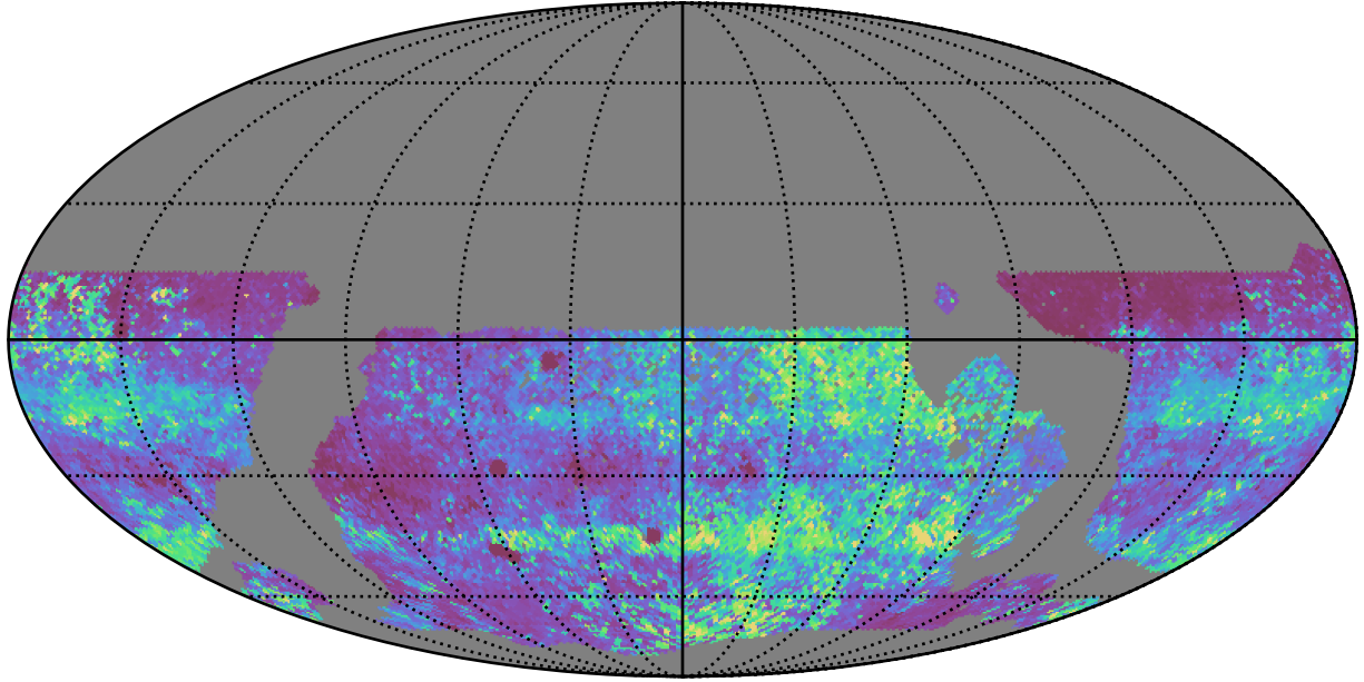
ddf_acor_sf10_lsf20_lsr10_v3.4_10yrs WFD zy bands: 75th Percentile Intranight Timespan
