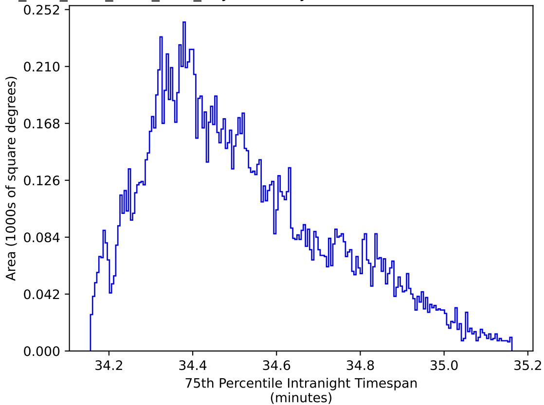
ddf_acor_sf10_lsf20_lsr10_v3.4_10yrs WFD zy bands: 75th Percentile Intranight Timespan
