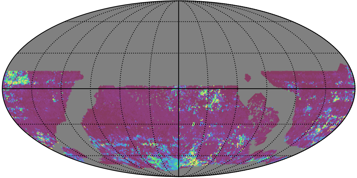
ddf_acor_sf10_lsf20_lsr10_v3.4_10yrs WFD z band: 75th Percentile Intranight Timespan
