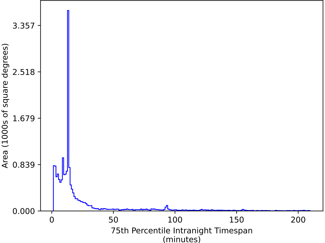
ddf_acor_sf10_lsf20_lsr10_v3.4_10yrs WFD z band: 75th Percentile Intranight Timespan
