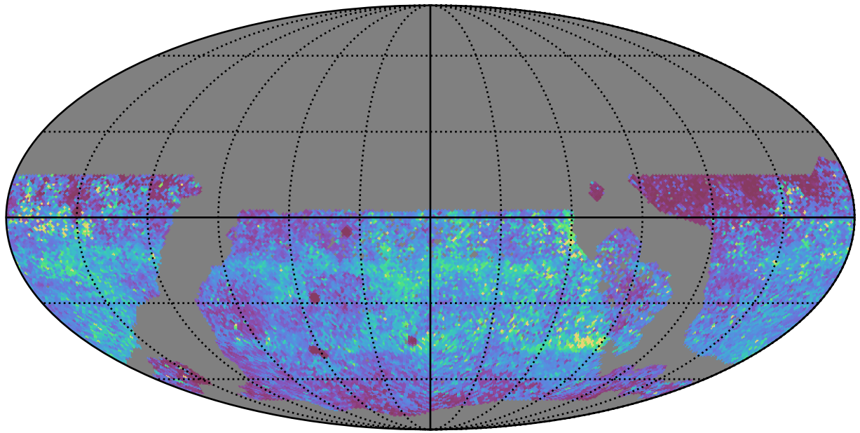
ddf_acor_sf10_lsf20_lsr10_v3.4_10yrs WFD y band: 75th Percentile Intranight Timespan
