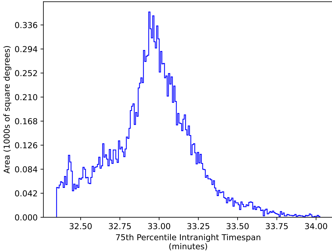
ddf_acor_sf10_lsf20_lsr10_v3.4_10yrs WFD y band: 75th Percentile Intranight Timespan
