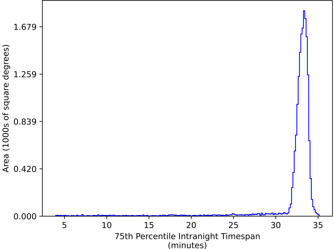
ddf_acor_sf10_lsf20_lsr10_v3.4_10yrs WFD ug bands: 75th Percentile Intranight Timespan
