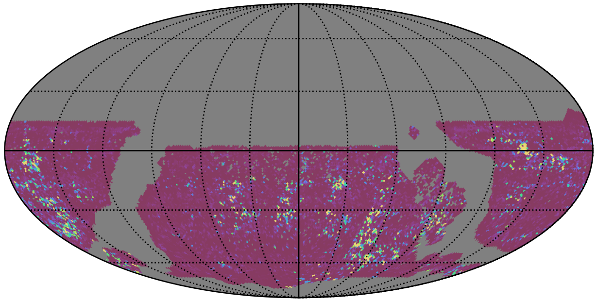
ddf_acor_sf10_lsf20_lsr10_v3.4_10yrs WFD u band: 75th Percentile Intranight Timespan
