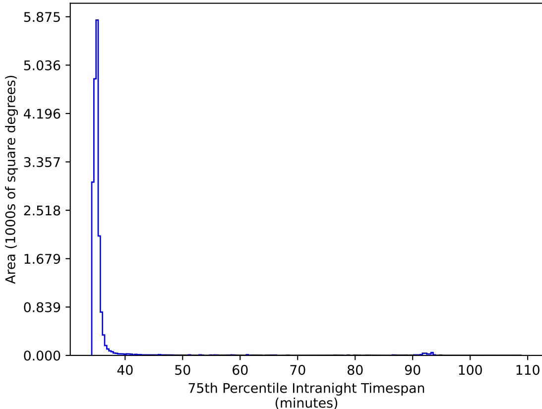
ddf_acor_sf10_lsf20_lsr10_v3.4_10yrs WFD ri bands: 75th Percentile Intranight Timespan
