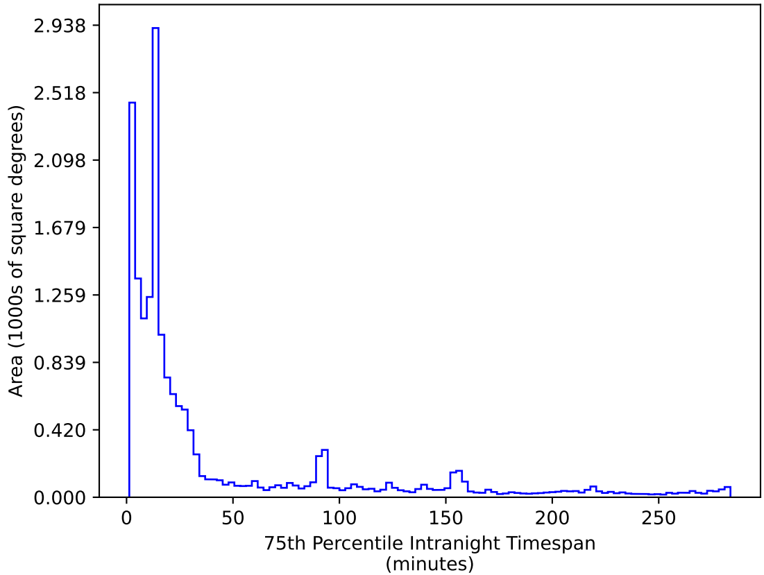
ddf_acor_sf10_ls20_lsr10_v3.4_10yrs WFD r band: 75th Percentile Intranight Timespan
