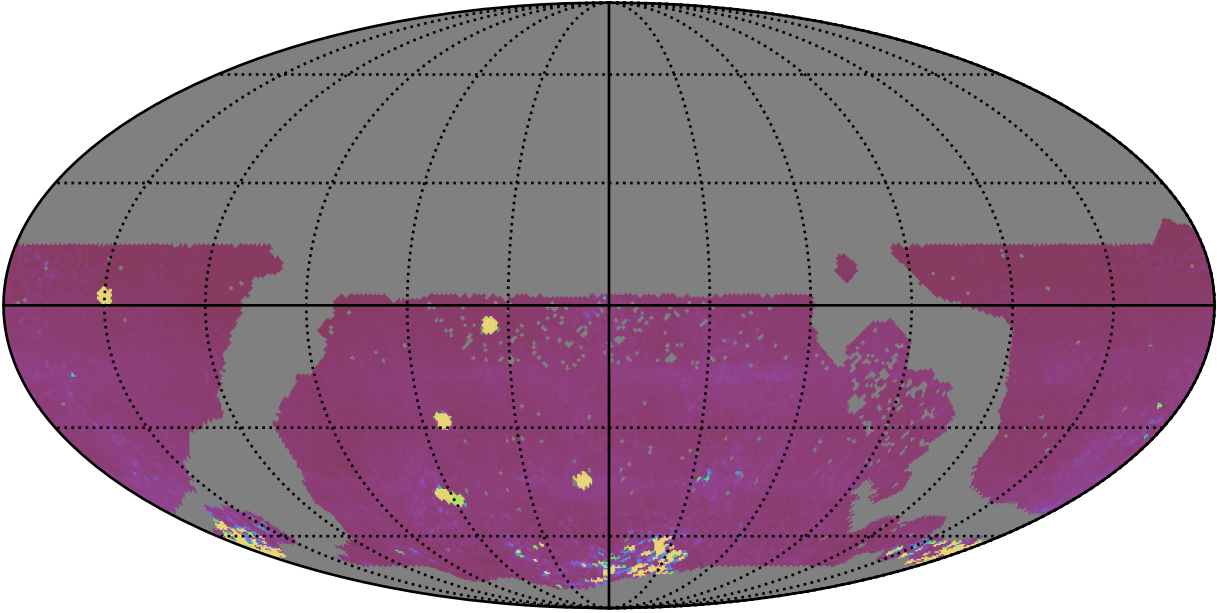
ddf_acor_sf10_lsf20_lsr10_v3.4_10yrs WFD iz bands: 75th Percentile Intranight Timespan
