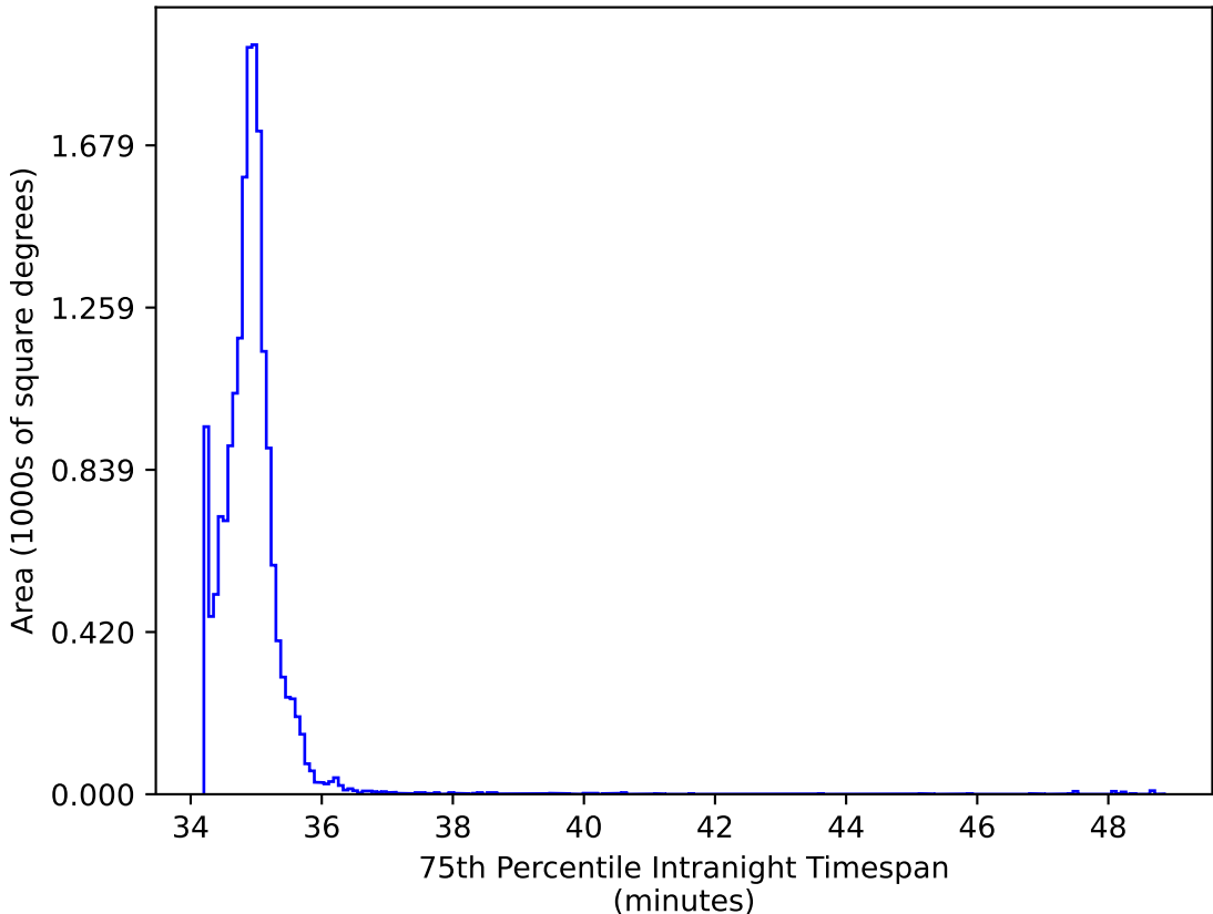
ddf_acor_sf10_lsf20_lsr10_v3.4_10yrs WFD iz bands: 75th Percentile Intranight Timespan
