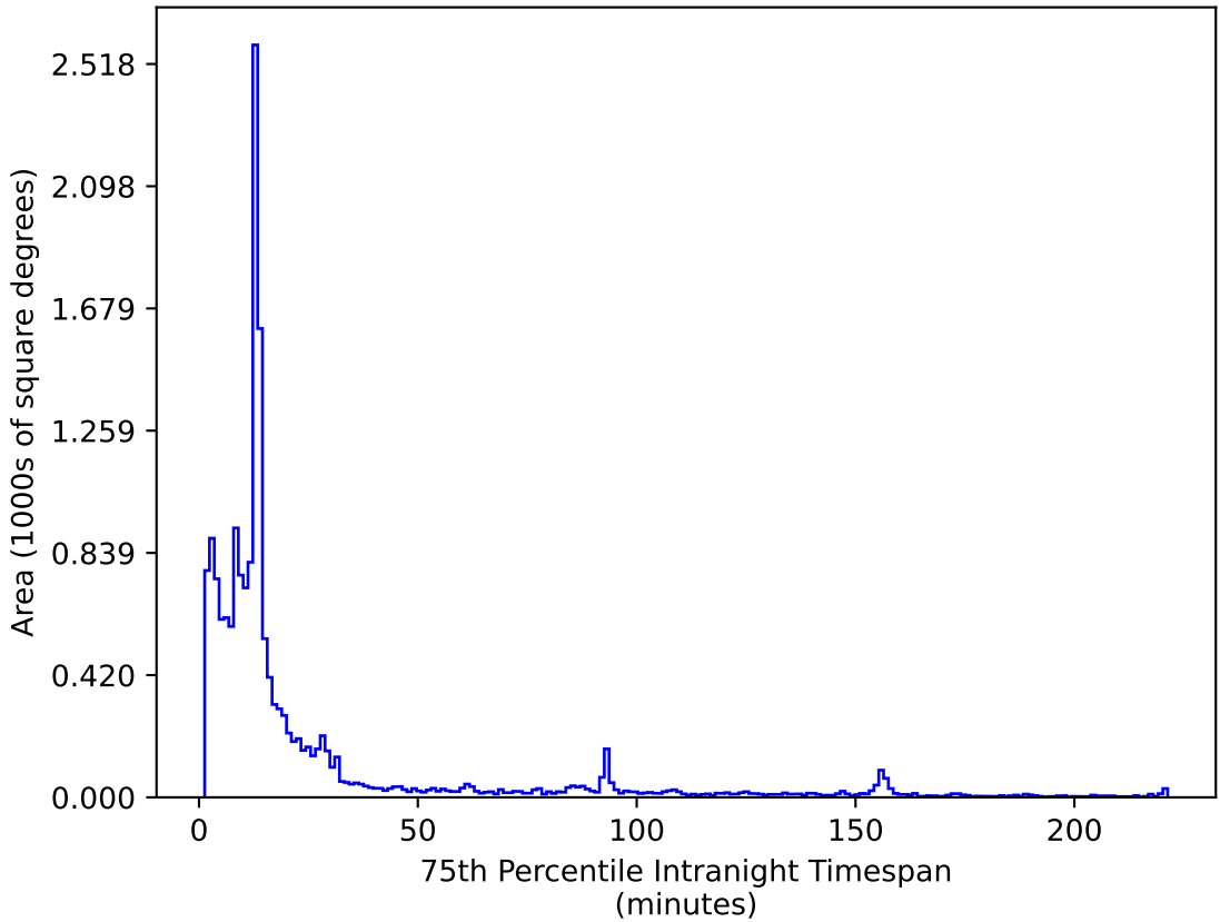
ddf_acor_sf10_lsf20_lsr10_v3.4_10yrs WFD i band: 75th Percentile Intranight Timespan
