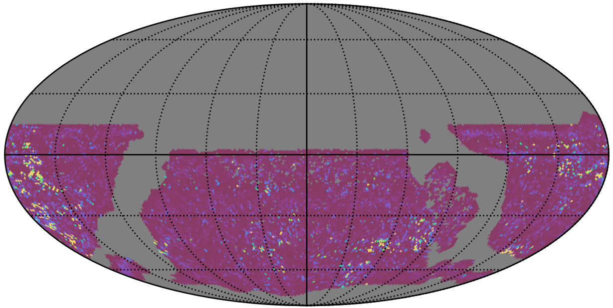
ddf_acor_sf10_lsf20_lsr10_v3.4_10yrs WFD g band: 75th Percentile Intranight Timespan
