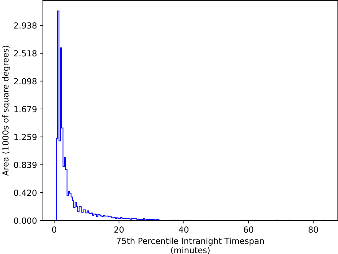
ddf_acor_sf10_lsf20_lsr10_v3.4_10yrs WFD g band: 75th Percentile Intranight Timespan
