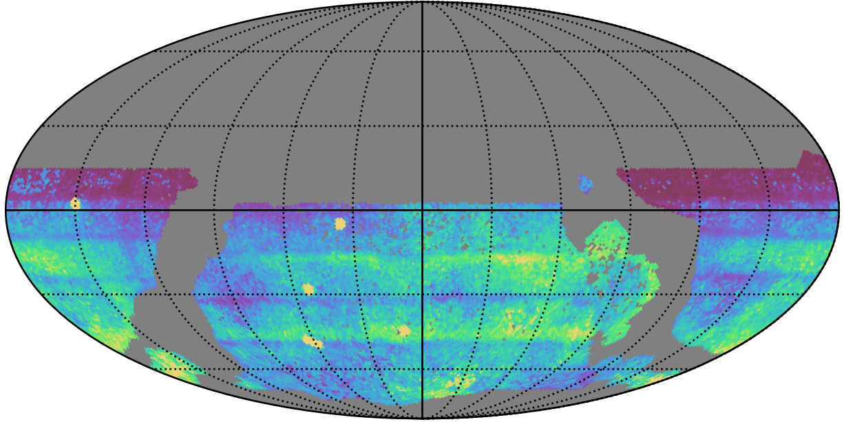
ddf_acor_sf10_lsf20_lsr10_v3.4_10yrs WFD all bands: 75th Percentile Intranight Timespan
