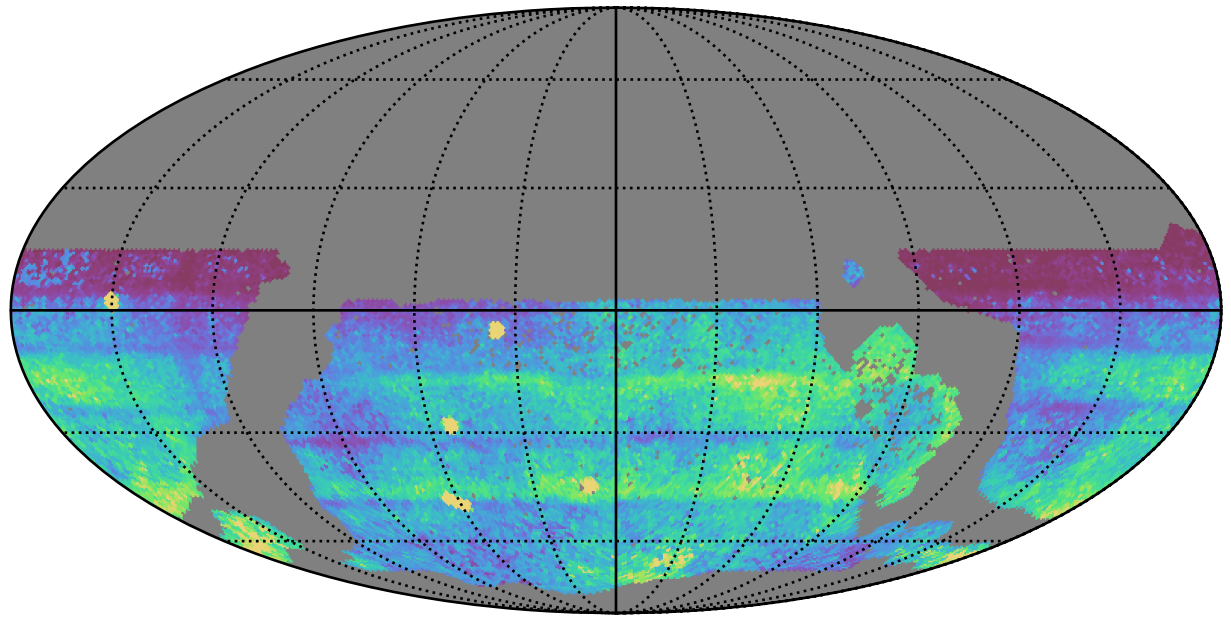
ddf_acor_sf10_lsf20_lsr10_v3.4_10yrs WFD: 75th Percentile Intranight Timespan
