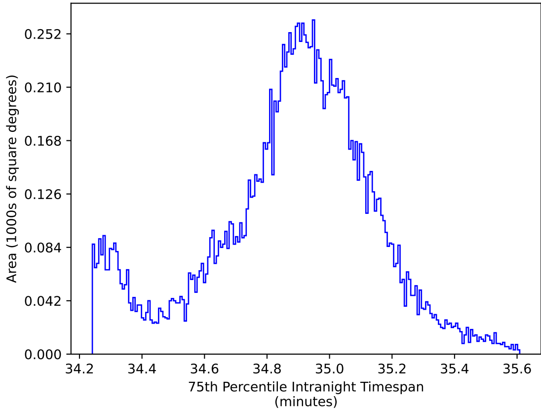
ddf_acor_sf10_lsf20_lsr10_v3.4_10yrs WFD: 75th Percentile Intranight Timespan
