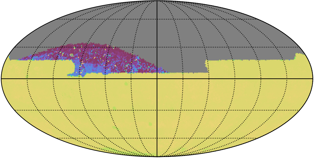
ddf_acor_sf10_lsf20_lsr10_v3.4_10yrs All sky zy bands: 75th Percentile Intranight Timespan
