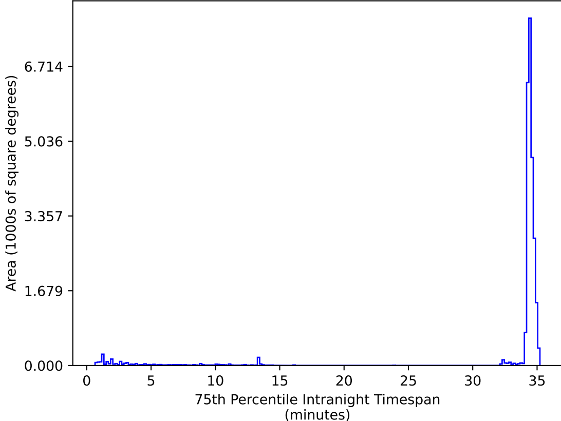
ddf_acor_sf10_lsf20_lsr10_v3.4_10yrs All sky zy bands: 75th Percentile Intranight Timespan
