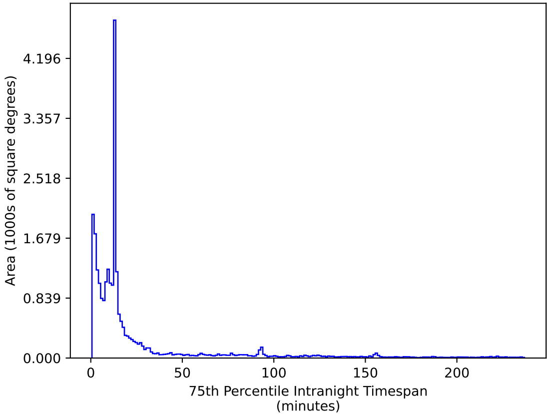
ddf_acor_sf10_lsf20_lsr10_v3.4_10yrs All sky z band: 75th Percentile Intranight Timespan
