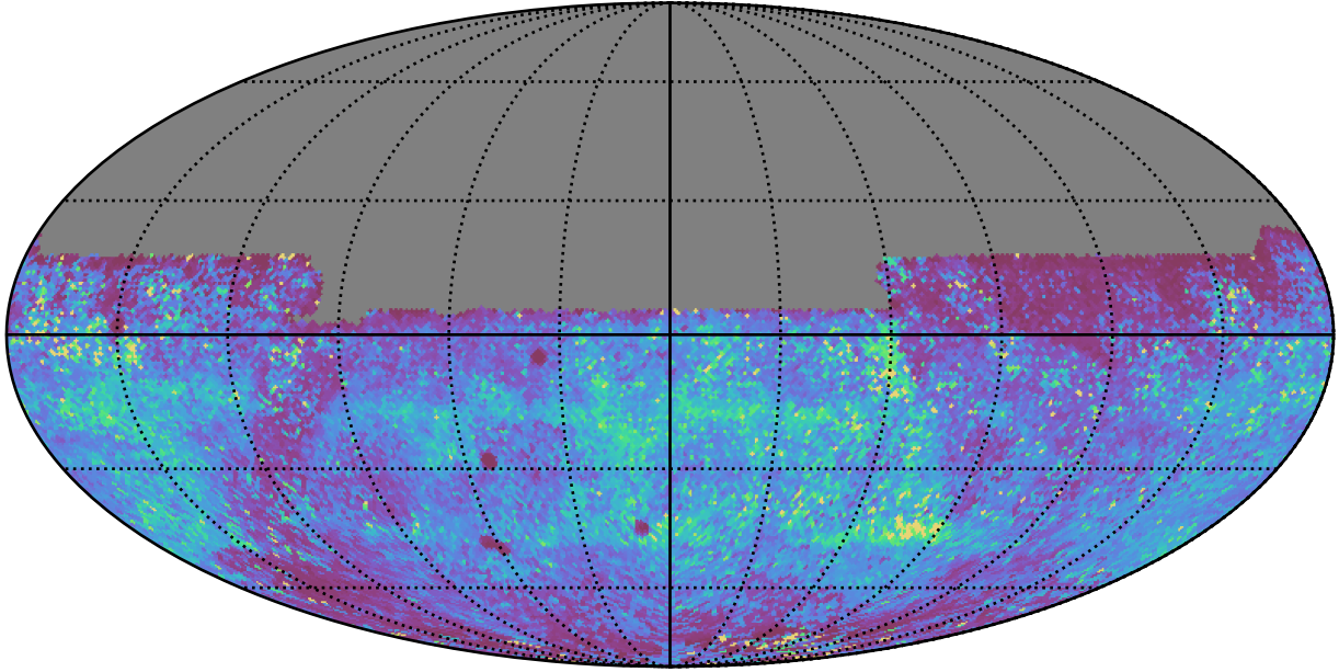
ddf_acor_sf10_lsf20_lsr10_v3.4_10yrs All sky y band: 75th Percentile Intranight Timespan
