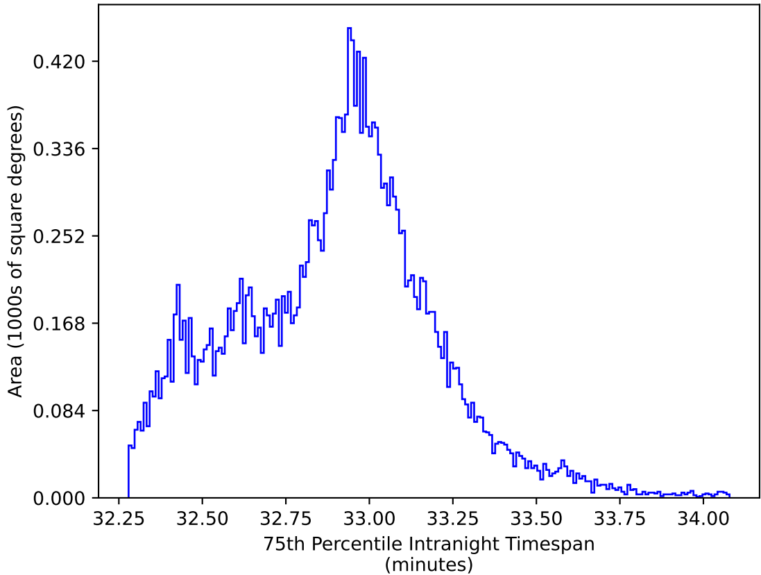
ddf_acor_sf10_lsf20_lsr10_v3.4_10yrs All sky y band: 75th Percentile Intranight Timespan
